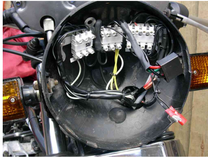
Connectionpoint – placed inside headlight
